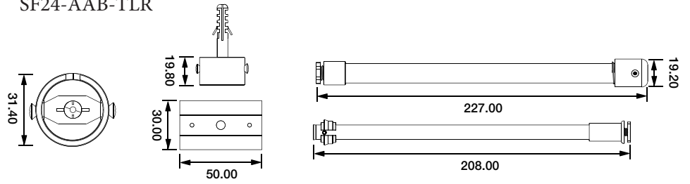
Aluminum alloy base Mounting Accessories Kit SF24-AAB-TLR
