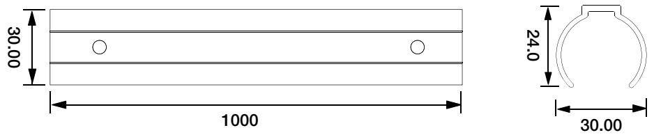
Mounting Plastic Channel PC24S01-T-100
