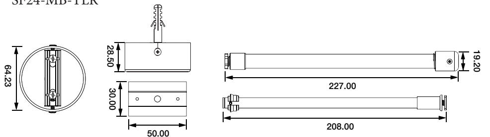
Metal base Mounting Accessories Kit
