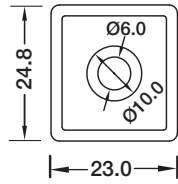
DIY Snap Connector DIY-SN-FR-16-D-01/02-A
