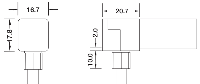
Bottom Entry Connector MJ-SF16-D5-S02SM MJ-SF16-D5-S03SFM
