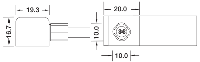
Side Entry Connector MJ-SF16-D5-S02SM MJ-SF16-D5-S03SFM
