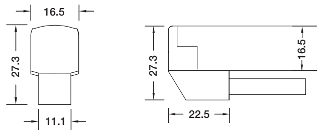
L Shape Entry Connector MJ-SF16-D5-L02SM MJ-SF16-D5-L03SFM
