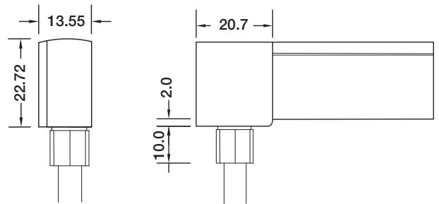
Bottom Entry Connector MJ-15-D4-S02SM MJ-15-D4-S03SFM
