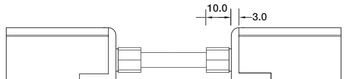
Jumper MJ-15-D4-D-JC
