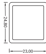
DIY Snap End Cap DIY-SN-END-17-D-01/02
